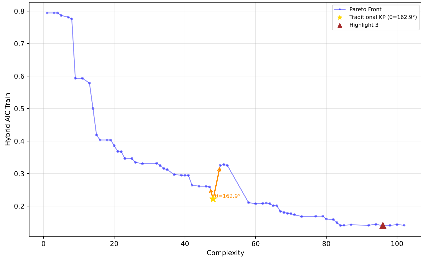
557_analcatdata_apnea1 - Run 1 - SVP - Hybrid AIC Train \lambda_1=0.00, \lambda_2=0.00, \lambda_3=0.00 | Difficulty: 1.00 | Method: hmr
