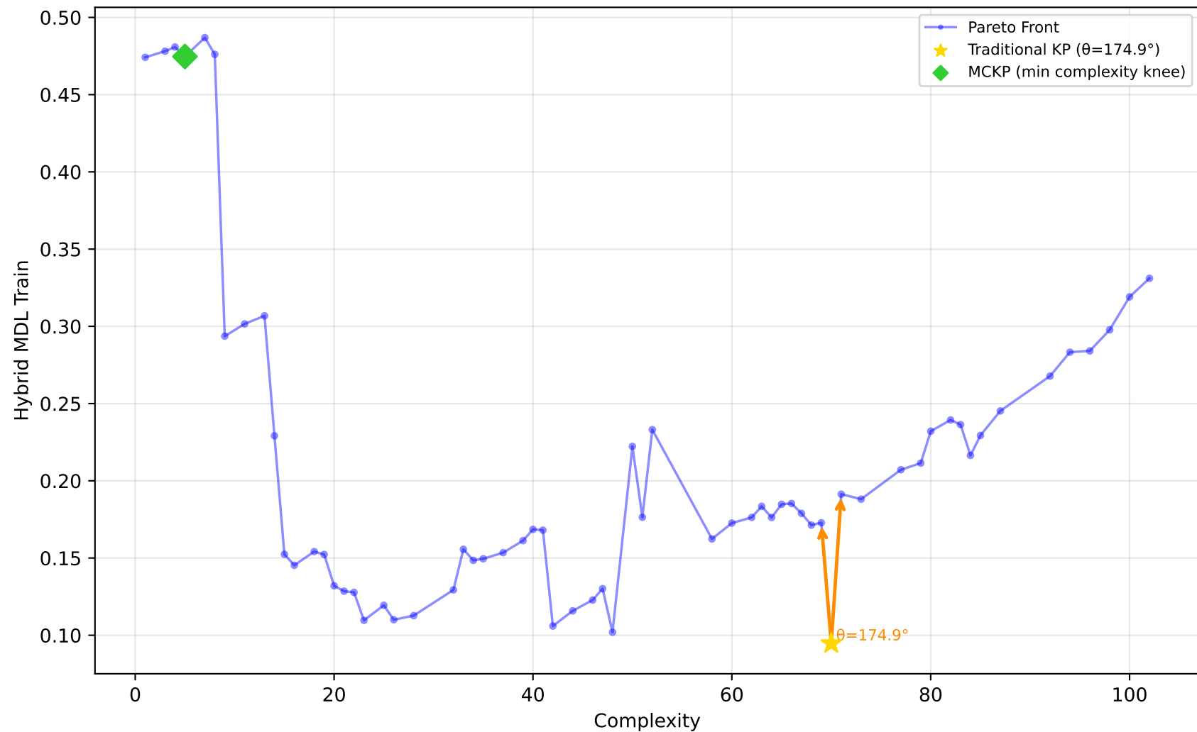
557_analcatdata_apnea1 - Run 1 - SVP - Hybrid MDL Train \lambda_1=0.00 , \lambda_2=0.00 , \lambda_3=0.00 | Difficulty: 1.00 | Method: hmr
