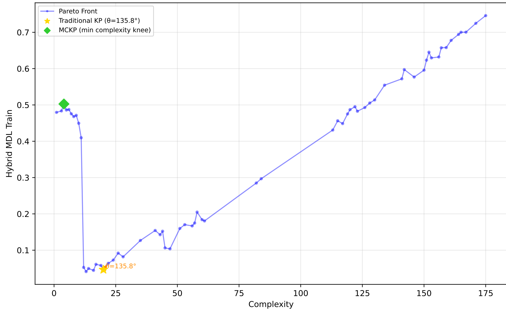
557_analcatdata_apnea1 - Run 20 - MVP - Hybrid MDL Train \lambda_1=0.00, \lambda_2=0.00, \lambda_3=0.00 | Difficulty: 1.00 | Method: hmr
