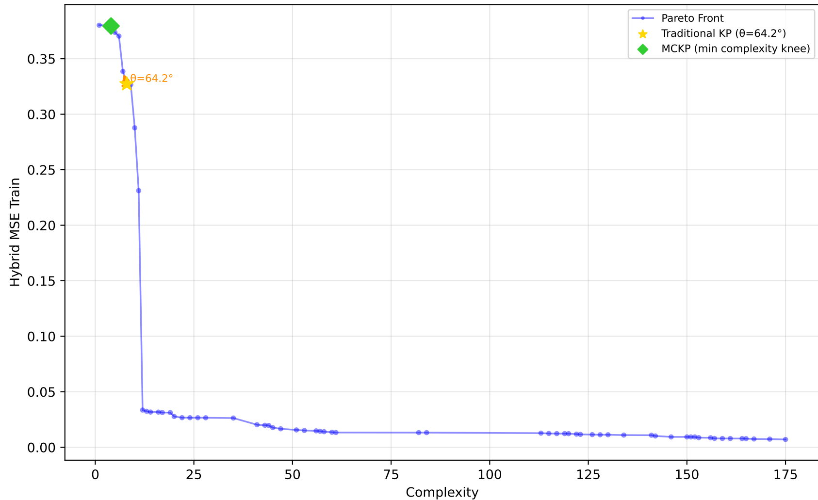
557_analcatdata_apnea1 - Run 20 - MVP - Hybrid MSE Train \lambda_1=0.00 , \lambda_2=0.00 , \lambda_3=0.00 | Difficulty: 1.00 | Method: hmr
