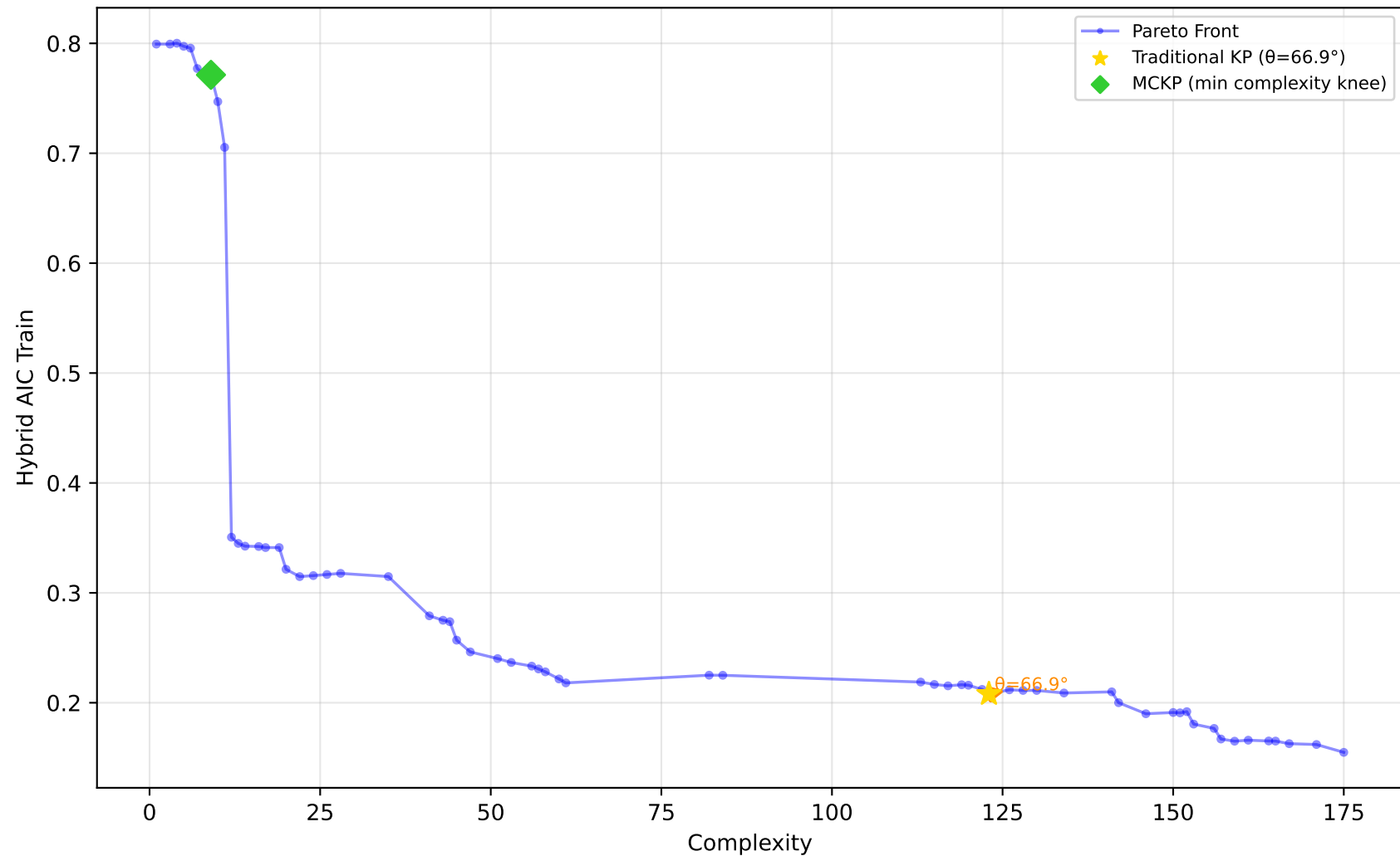
557_analcatdata_apnea1 - Run 20 - SVP - Hybrid AIC Train \lambda_1=0.00 , \lambda_2=0.00 , \lambda_3=0.00 | Difficulty: 1.00 | Method: hmr
