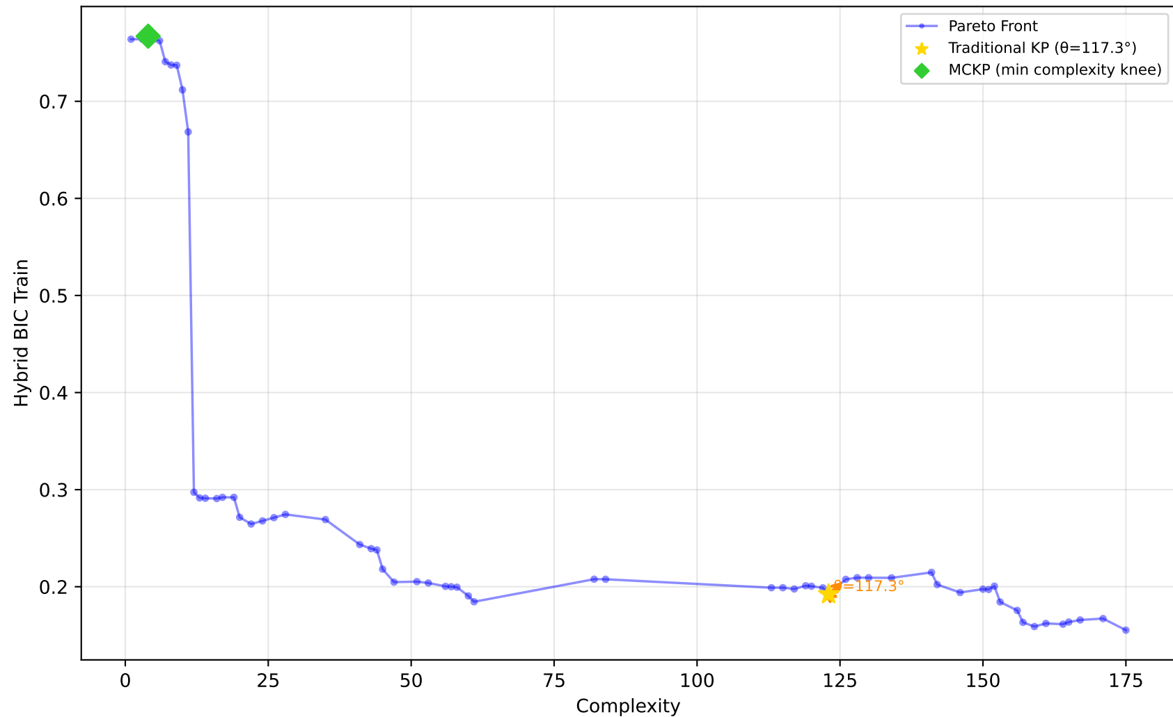
557_analcatdata_apnea1 - Run 20 - SVP - Hybrid BIC Train \lambda_1=0.00, \lambda_2=0.00, \lambda_3=0.00 | Difficulty: 1.00 | Method: hmr
