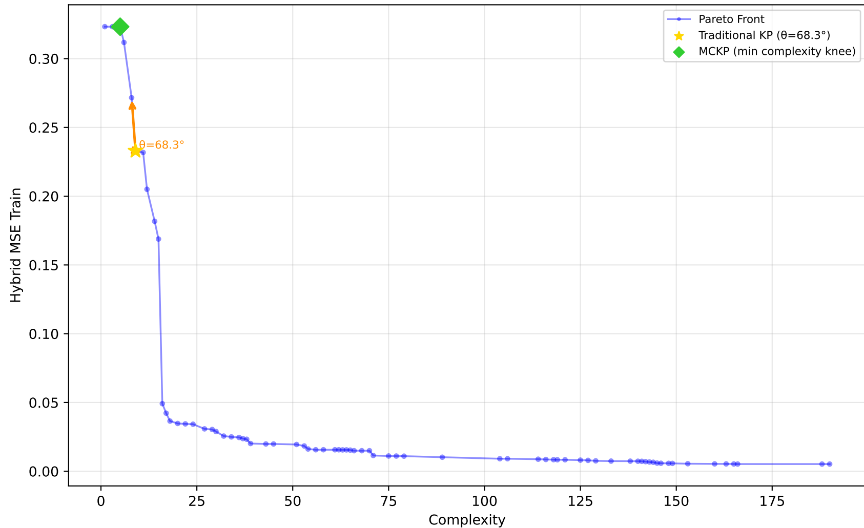
557_analcatdata_apnea1 - Run 21 - MVP - Hybrid MSE Train \lambda_1=0.00, \lambda_2=0.00, \lambda_3=0.00 | Difficulty: 0.81 | Method: hmr
