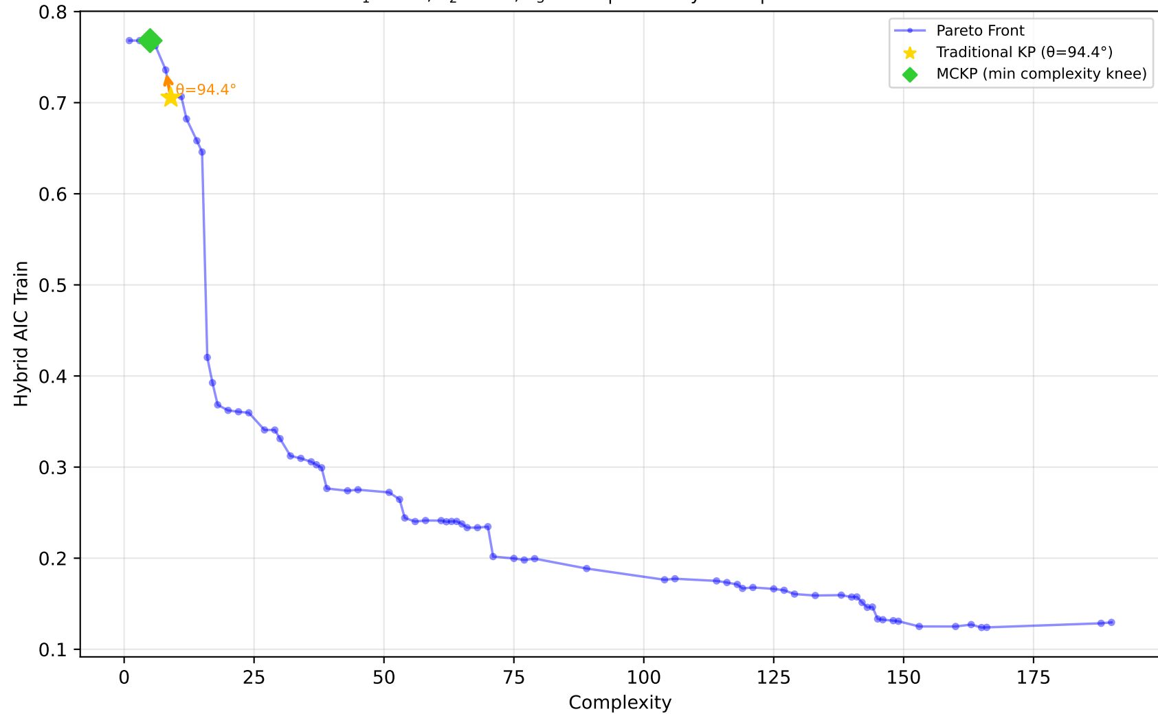
557_analcatdata_apnea1 - Run 21 - SVP - Hybrid AIC Train \lambda_1=0.00, \lambda_2=0.00, \lambda_3=0.00 | Difficulty: 0.81 | Method: hmr
