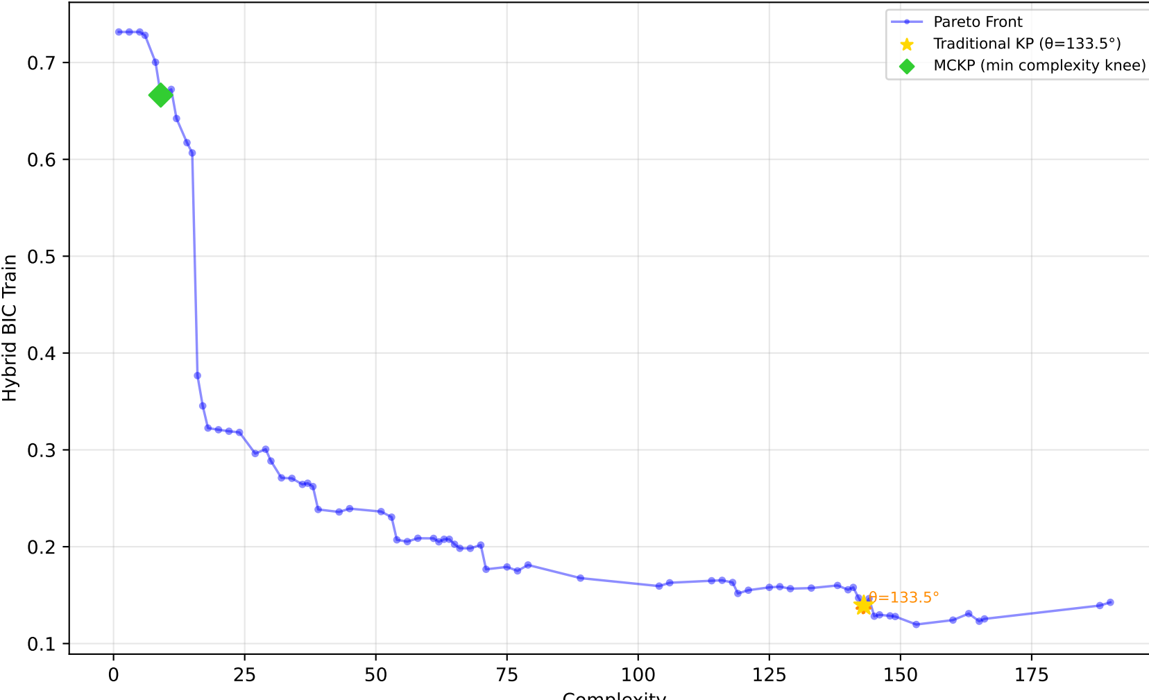
557_analcatdata_apnea1 - Run 21 - SVP - Hybrid BIC Train \lambda_1=0.00 , \lambda_2=0.00 , \lambda_3=0.00 | Difficulty: 0.81 | Method: hmr
