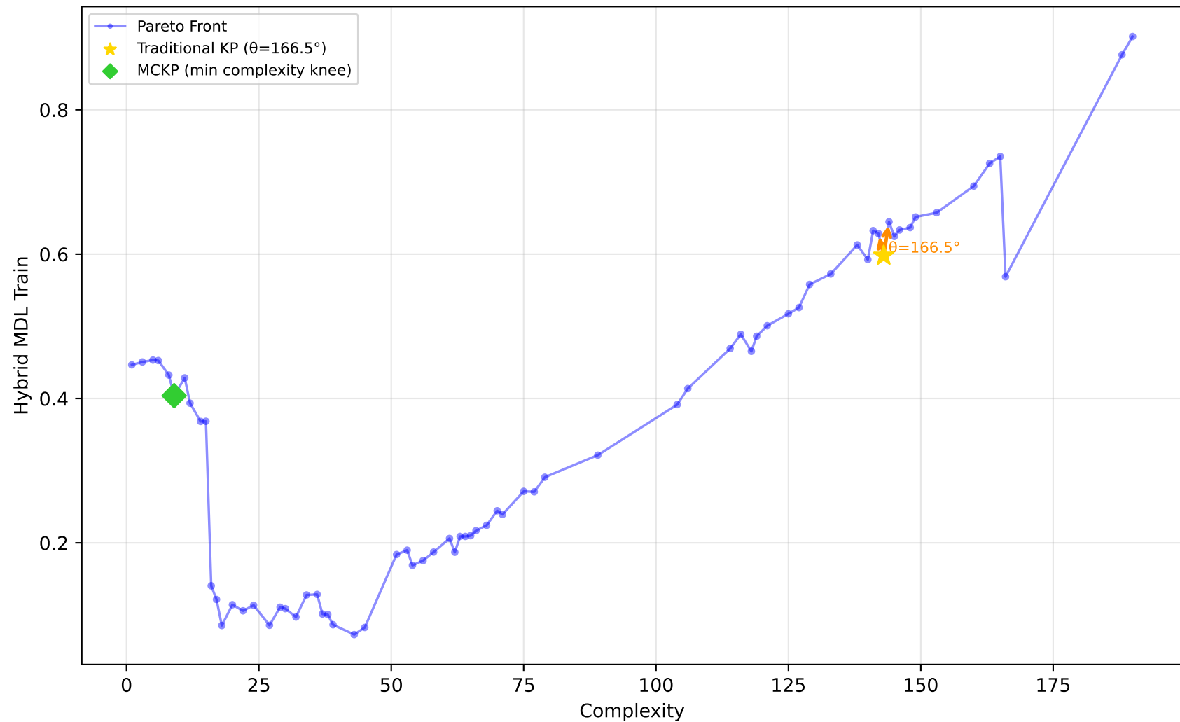
557_analcatdata_apnea1 - Run 21 - SVP - Hybrid MDL Train \lambda_1=0.00, \lambda_2=0.00, \lambda_3=0.00 | Difficulty: 0.81 | Method: hmr
