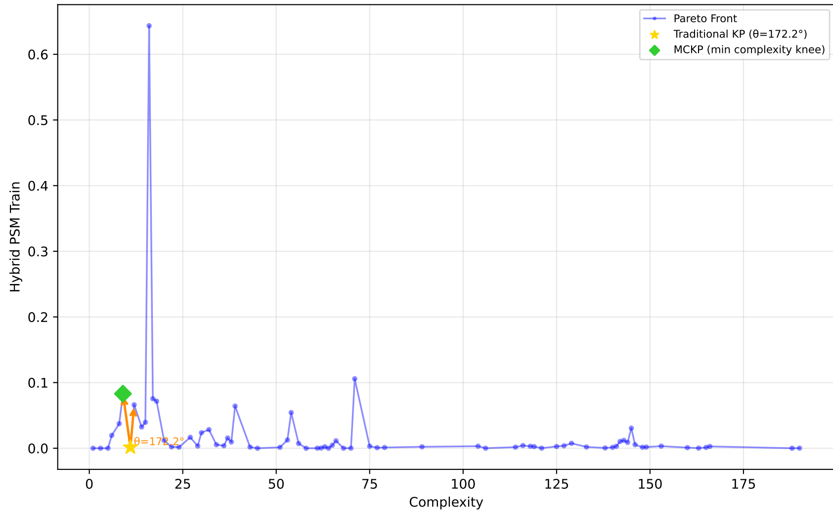
557_analcatdata_apnea1 - Run 21 - SVP - Hybrid PSM Train \lambda_1=0.00, \lambda_2=0.00, \lambda_3=0.00 | Difficulty: 0.81 | Method: hmr
