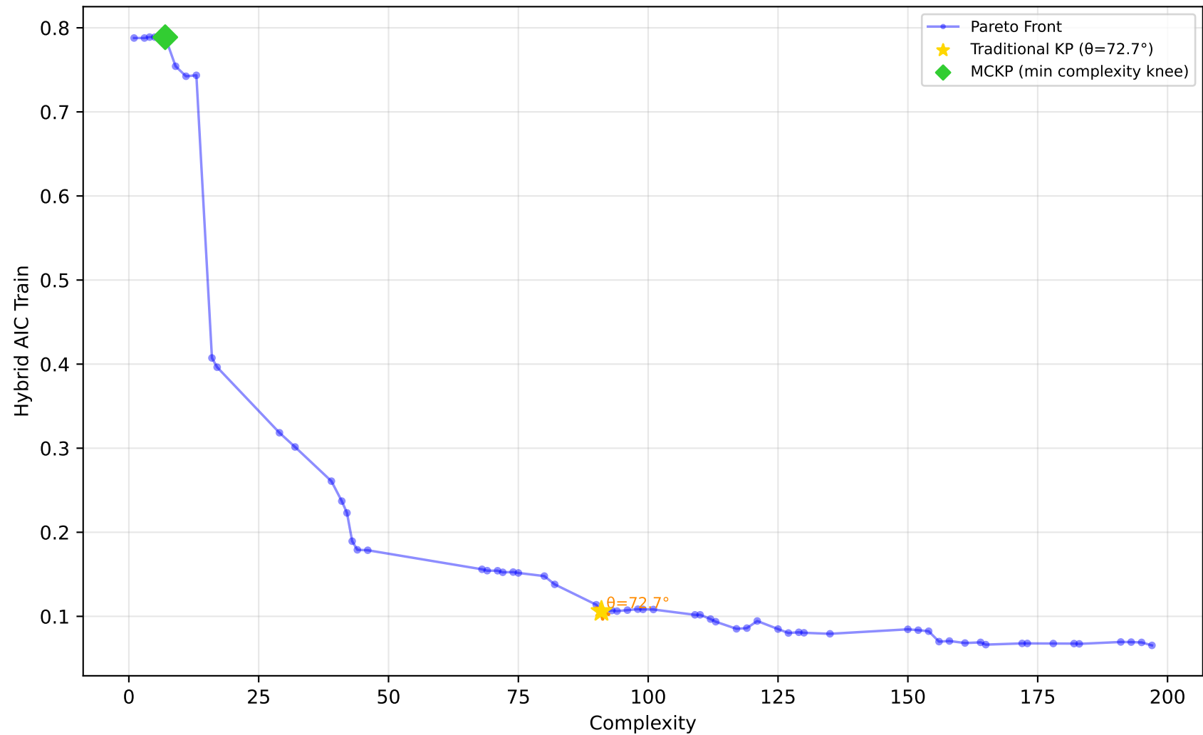
557_analcatdata_apnea1 - Run 22 - MVP - Hybrid AIC Train \lambda_1=0.00 , \lambda_2=0.00 , \lambda_3=0.00 | Difficulty: 1.00 | Method: hmr
