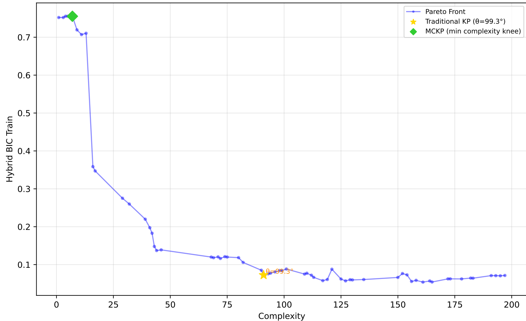
557_analcatdata_apnea1 - Run 22 - MVP - Hybrid BIC Train \lambda_1=0.00, \lambda_2=0.00, \lambda_3=0.00 | Difficulty: 1.00 | Method: hmr
