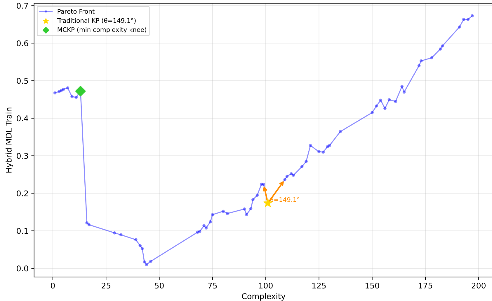
557_analcatdata_apnea1 - Run 22 - MVP - Hybrid MDL Train \lambda_1=0.00, \lambda_2=0.00, \lambda_3=0.00 | Difficulty: 1.00 | Method: hmr
