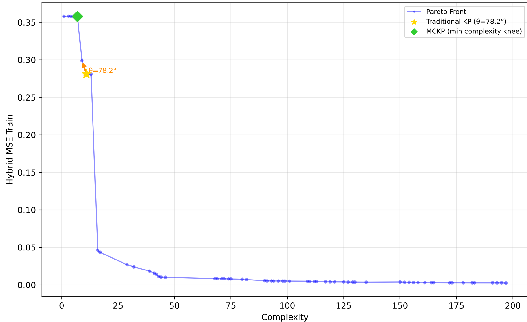
557_analcatdata_apnea1 - Run 22 - MVP - Hybrid MSE Train \lambda_1=0.00, \lambda_2=0.00, \lambda_3=0.00 | Difficulty: 1.00 | Method: hmr
