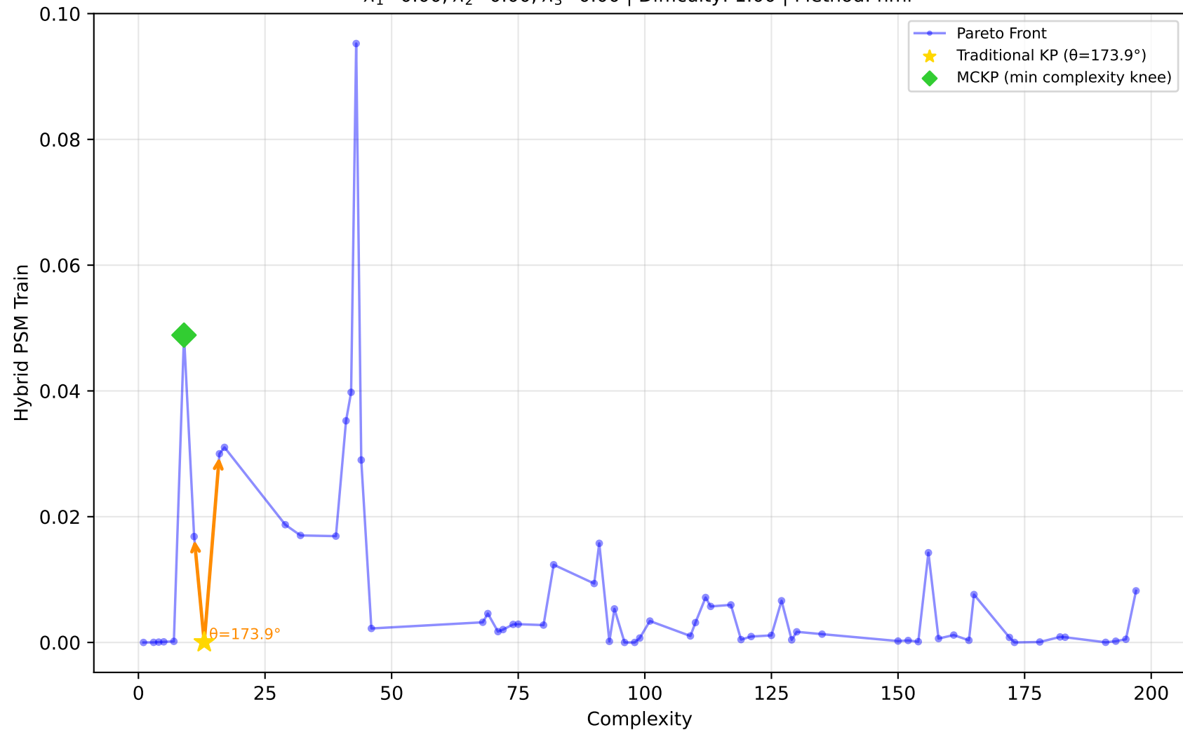
557_analcatdata_apnea1 - Run 22 - MVP - Hybrid PSM Train \lambda_1=0.00 , \lambda_2=0.00 , \lambda_3=0.00 | Difficulty: 1.00 | Method: hmr
