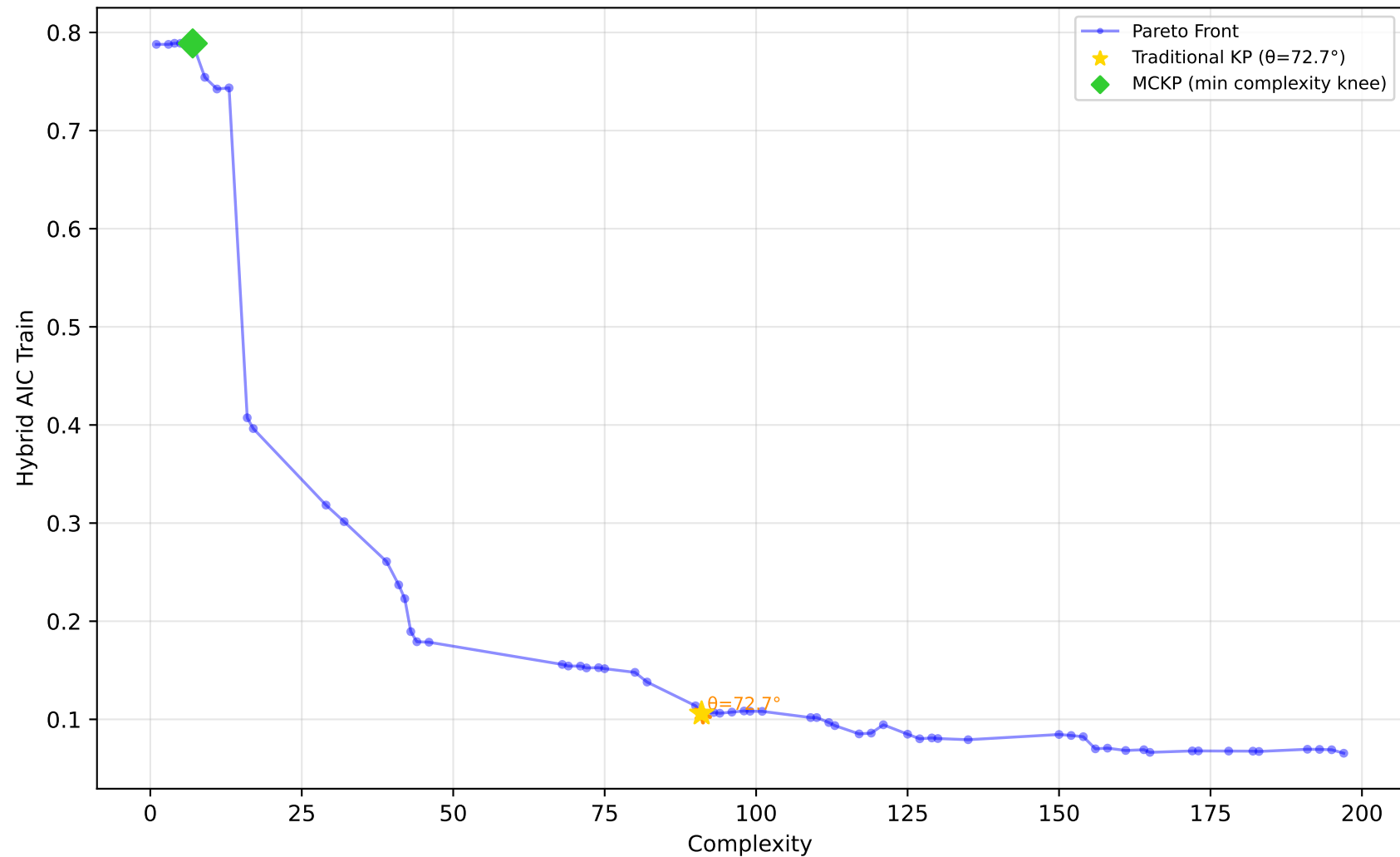
557_analcatdata_apnea1 - Run 22 - SVP - Hybrid AIC Train \lambda_1=0.00, \lambda_2=0.00, \lambda_3=0.00 | Difficulty: 1.00 | Method: hmr
