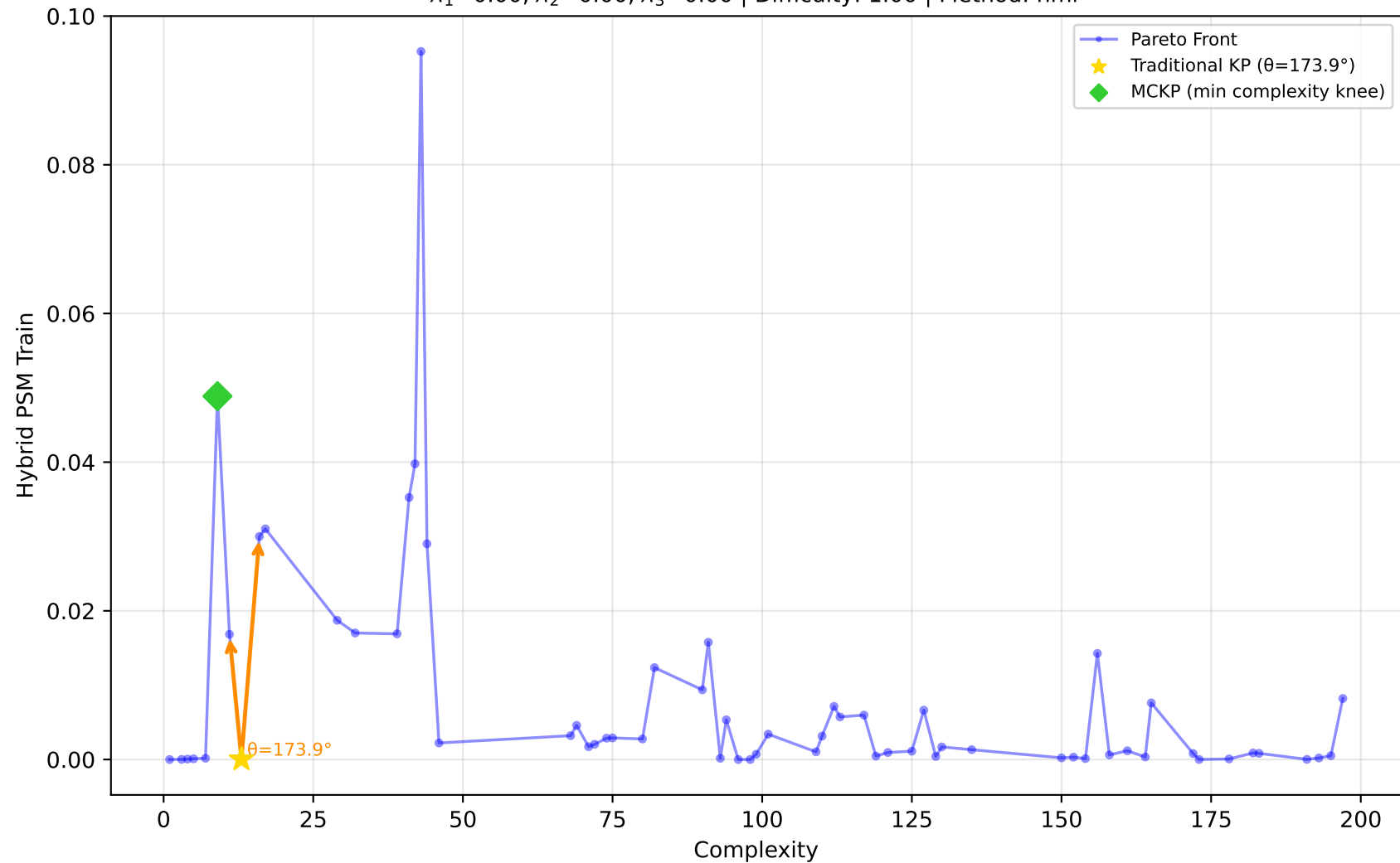
557_analcatdata_apnea1 - Run 22 - SVP - Hybrid PSM Train \lambda_1=0.00, \lambda_2=0.00, \lambda_3=0.00 | Difficulty: 1.00 | Method: hmr
