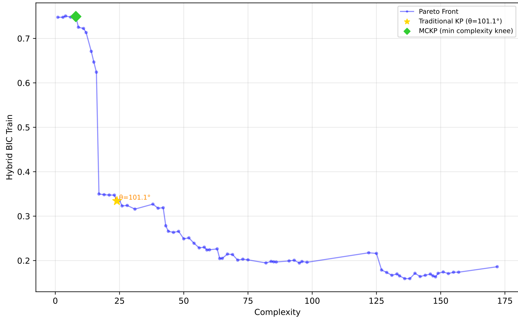
557_analcatdata_apnea1 - Run 23 - MVP - Hybrid BIC Train \lambda_1=0.00, \lambda_2=0.00, \lambda_3=0.00 | Difficulty: 1.00 | Method: hmr
