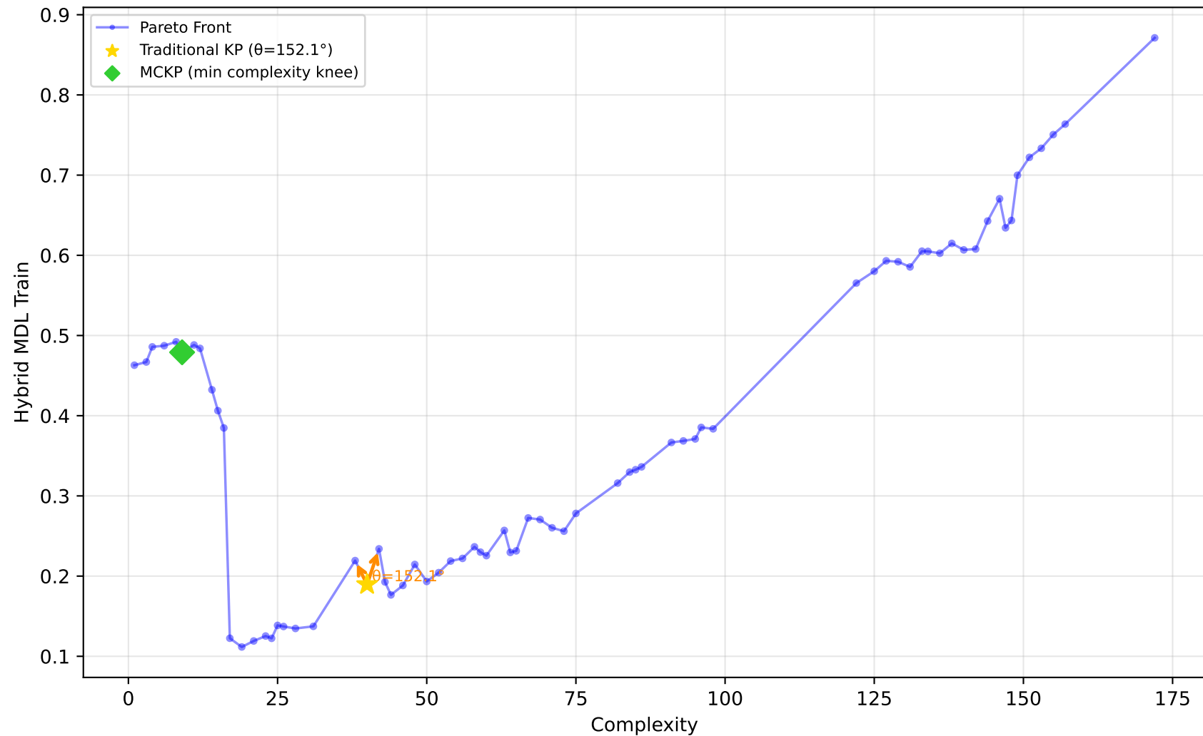
557_analcatdata_apnea1 - Run 23 - MVP - Hybrid MDL Train \lambda_1=0.00, \lambda_2=0.00, \lambda_3=0.00 | Difficulty: 1.00 | Method: hmr
