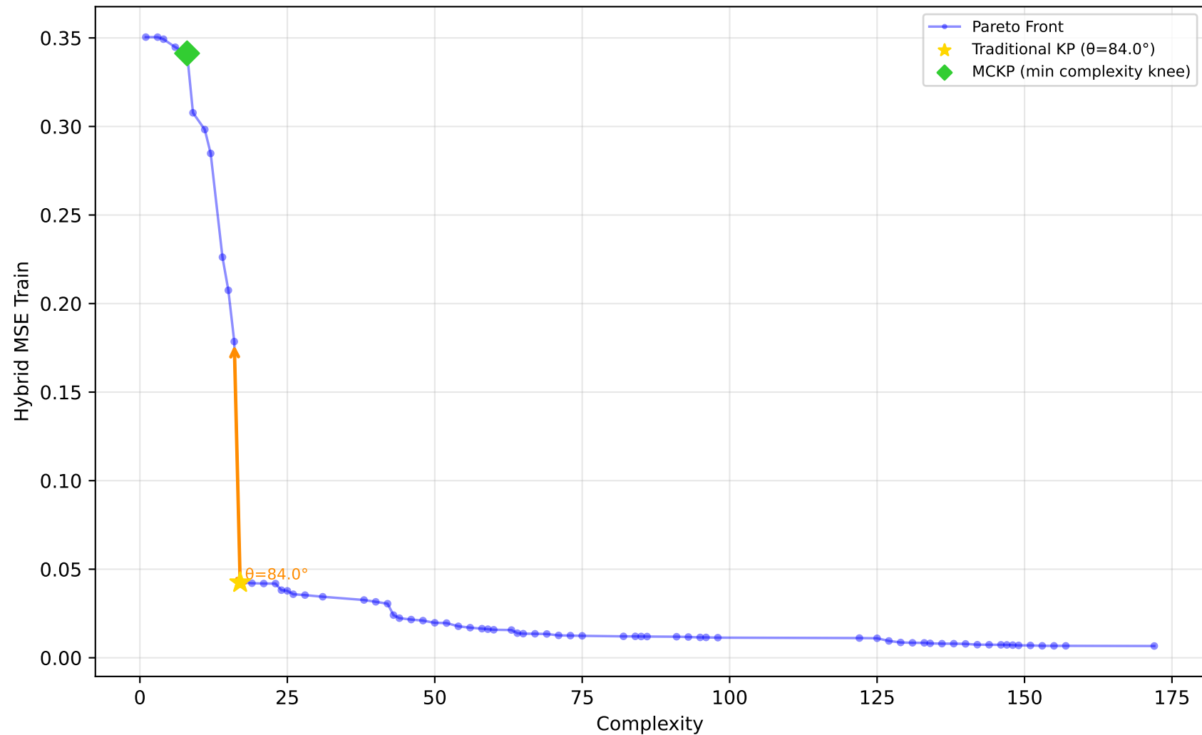
557_analcatdata_apnea1 - Run 23 - SVP - Hybrid MSE Train \lambda_1=0.00, \lambda_2=0.00, \lambda_3=0.00 | Difficulty: 1.00 | Method: hmr
