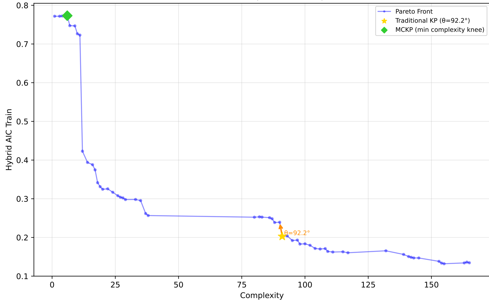
557_analcatdata_apnea1 - Run 24 - MVP - Hybrid AIC Train \lambda_1=0.00, \lambda_2=0.00, \lambda_3=0.00 | Difficulty: 0.89 | Method: hmr
