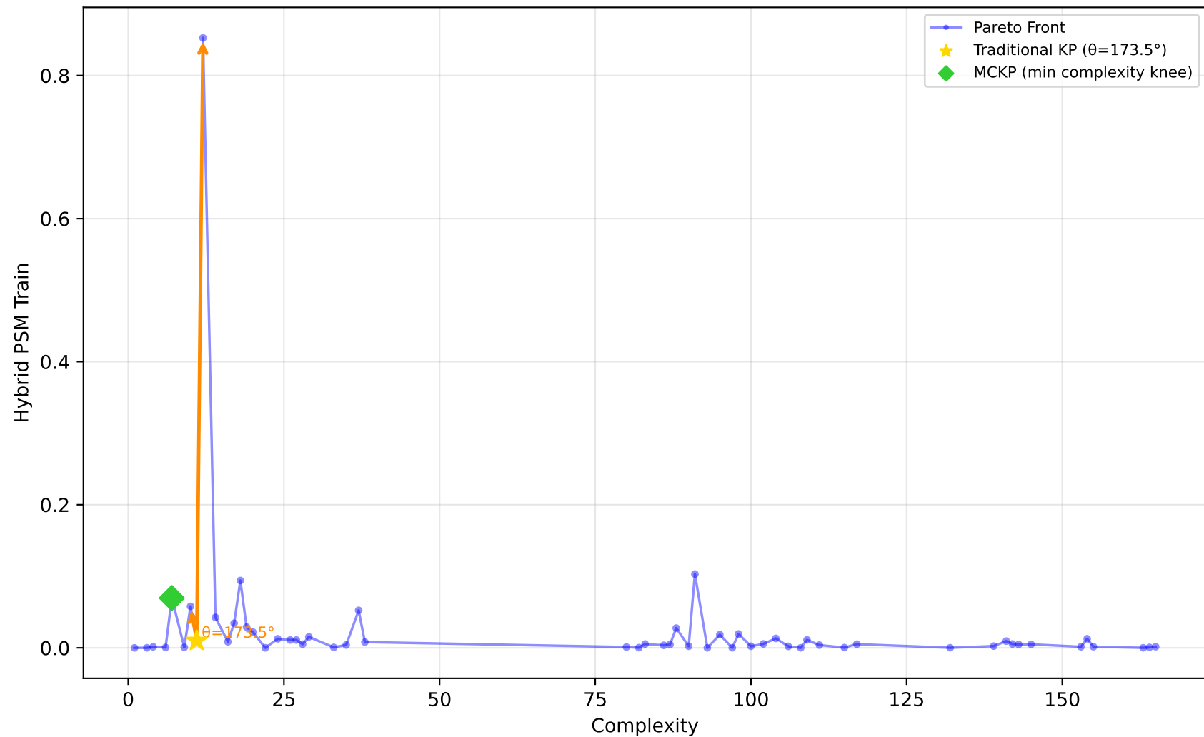
557_analcatdata_apnea1 - Run 24 - MVP - Hybrid PSM Train \lambda_1=0.00, \lambda_2=0.00, \lambda_3=0.00 | Difficulty: 0.89 | Method: hmr
