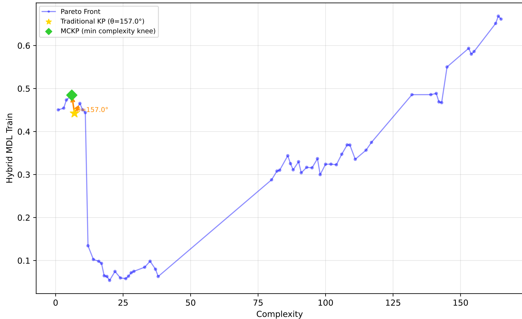
557_analcatdata_apnea1 - Run 24 - SVP - Hybrid MDL Train \lambda_1=0.00, \lambda_2=0.00, \lambda_3=0.00 | Difficulty: 0.89 | Method: hmr
