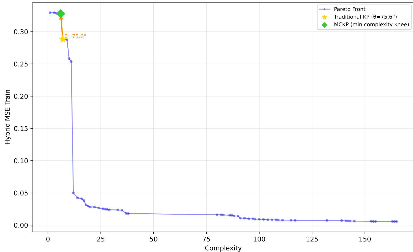
557_analcatdata_apnea1 - Run 24 - SVP - Hybrid MSE Train \lambda_1=0.00 , \lambda_2=0.00 , \lambda_3=0.00 | Difficulty: 0.89 | Method: hmr
