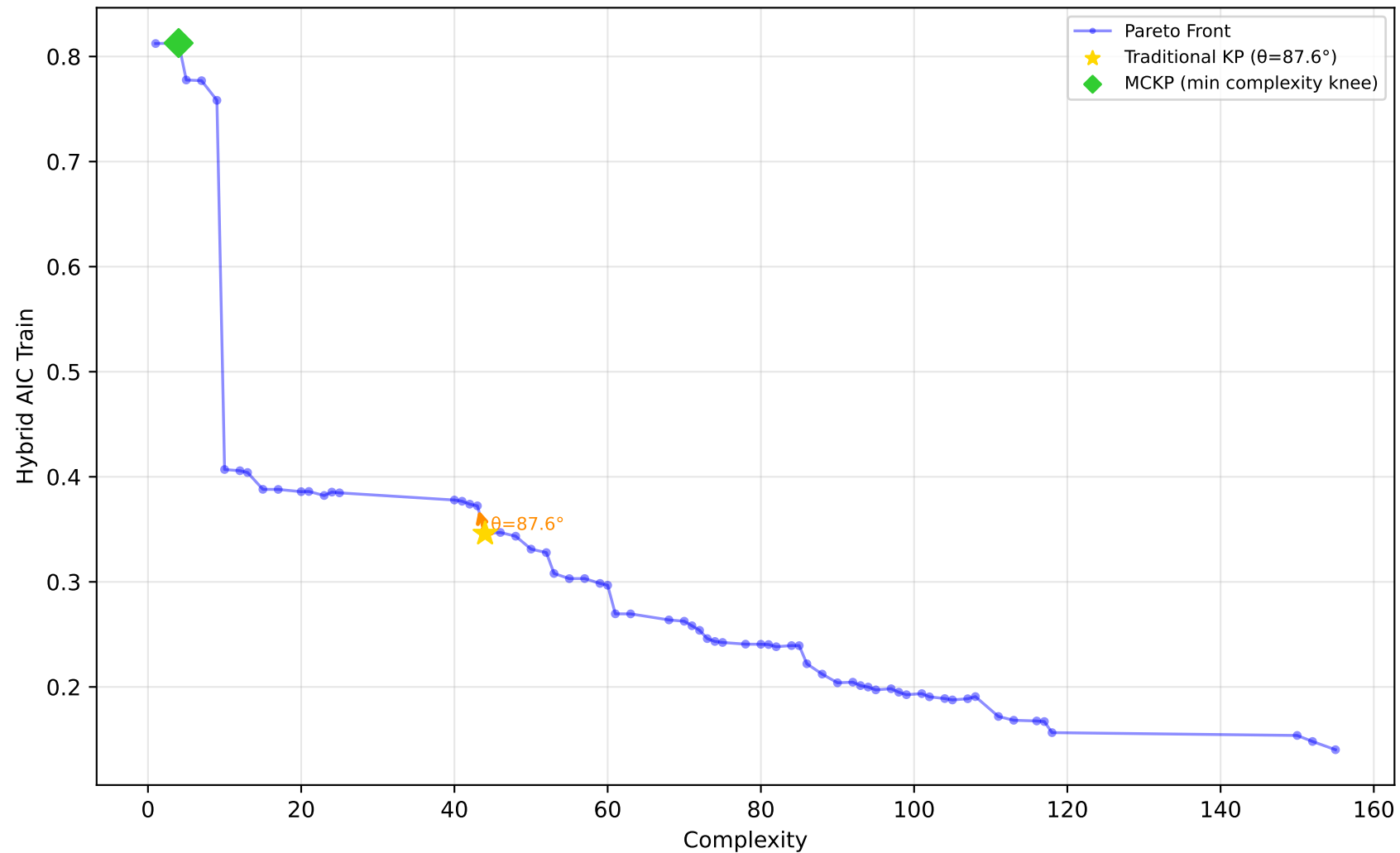
557_analcatdata_apnea1 - Run 25 - MVP - Hybrid AIC Train \lambda_1=0.00, \lambda_2=0.00, \lambda_3=0.00 | Difficulty: 1.00 | Method: hmr
