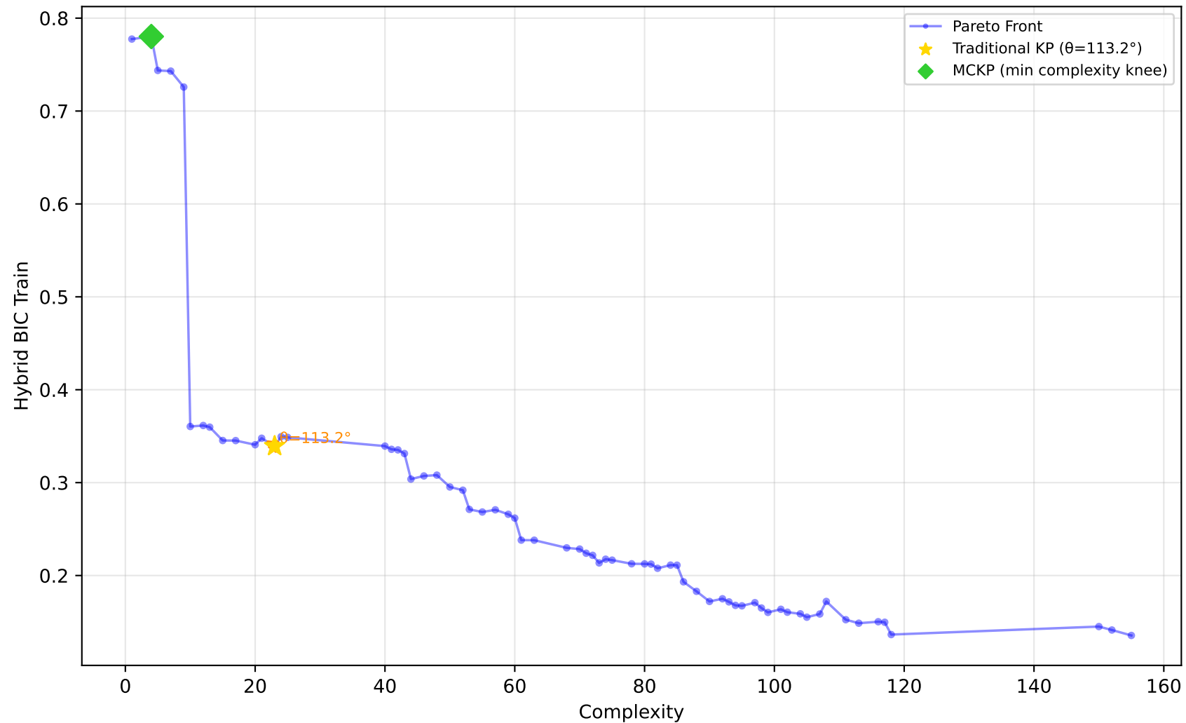
557_analcatdata_apnea1 - Run 25 - MVP - Hybrid BIC Train \lambda_1=0.00, \lambda_2=0.00, \lambda_3=0.00 | Difficulty: 1.00 | Method: hmr
