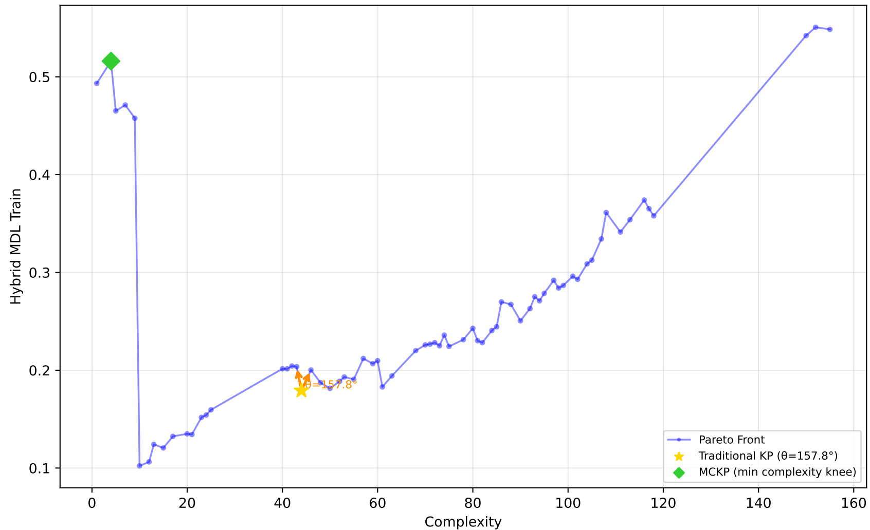
557_analcatdata_apnea1 - Run 25 - SVP - Hybrid MDL Train \lambda_1=0.00, \lambda_2=0.00, \lambda_3=0.00 | Difficulty: 1.00 | Method: hmr
