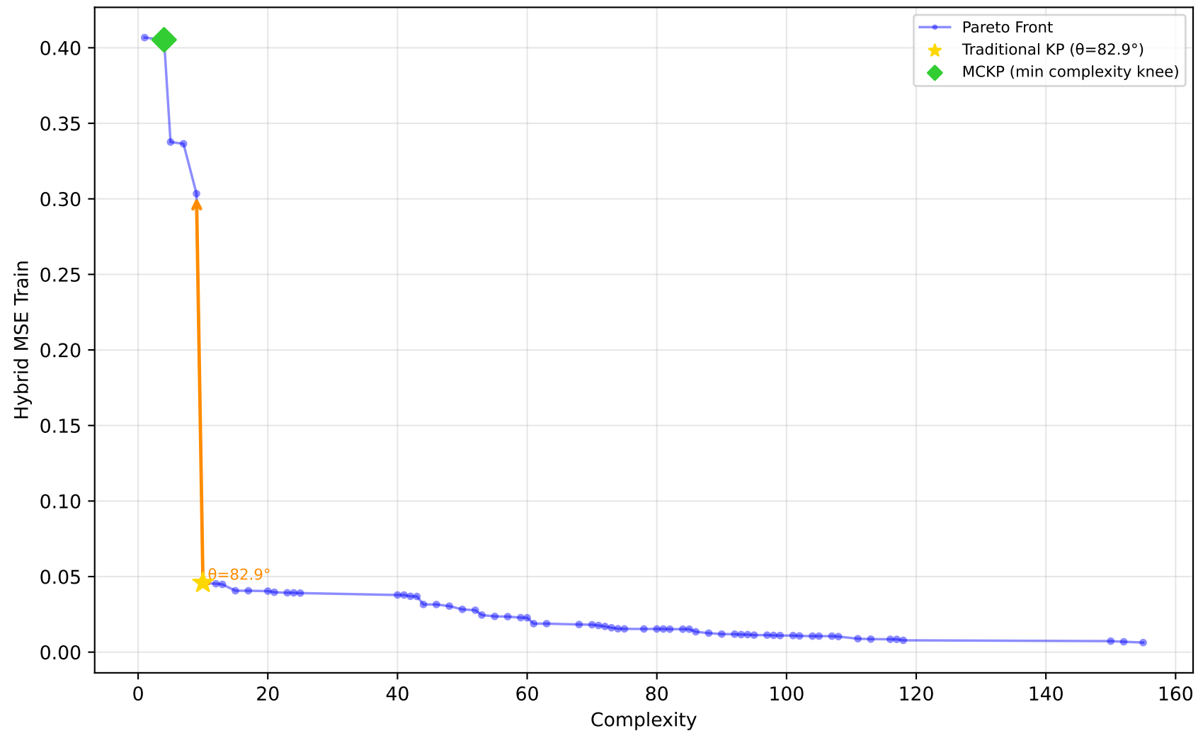
557_analcatdata_apnea1 - Run 25 - SVP - Hybrid MSE Train \lambda_1=0.00 , \lambda_2=0.00 , \lambda_3=0.00 | Difficulty: 1.00 | Method: hmr
