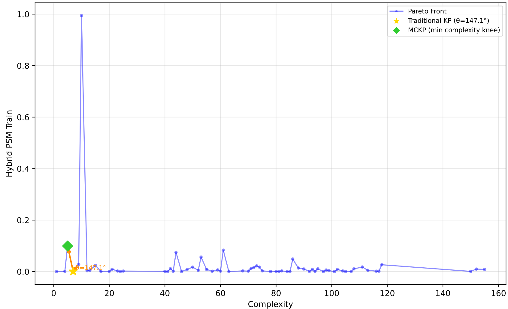
557_analcatdata_apnea1 - Run 25 - SVP - Hybrid PSM Train \lambda_1=0.00, \lambda_2=0.00, \lambda_3=0.00 | Difficulty: 1.00 | Method: hmr
