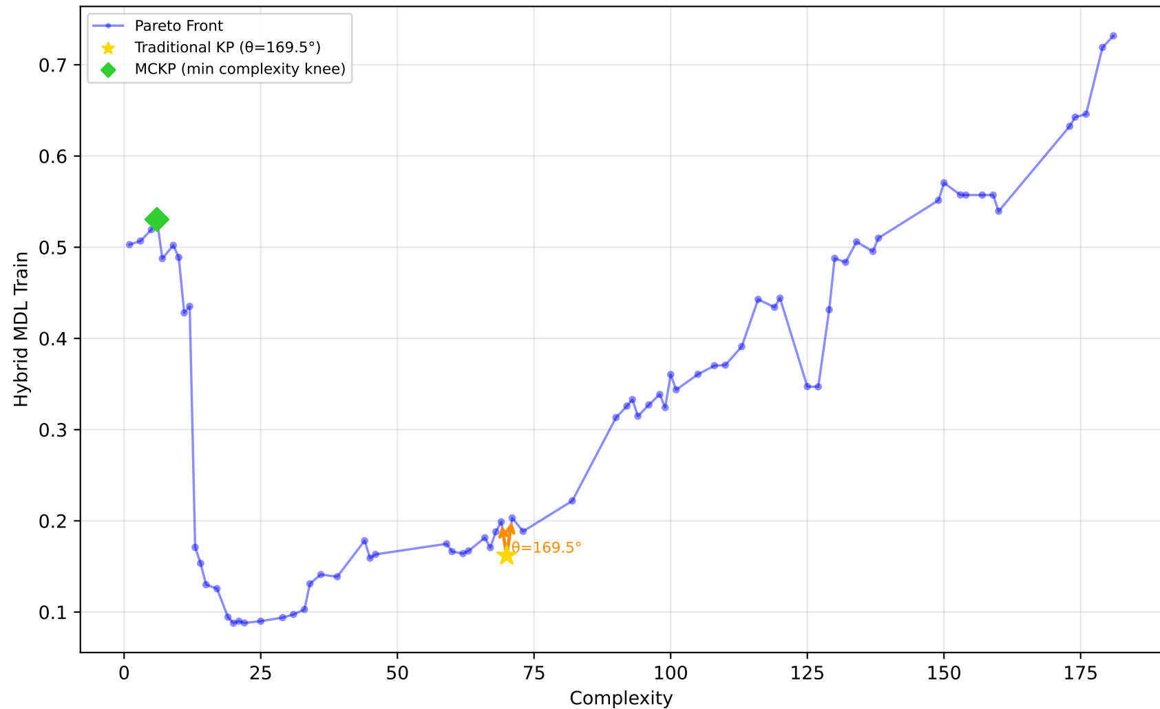
557_analcatdata_apnea1 - Run 26 - MVP - Hybrid MDL Train \lambda_1=0.00, \lambda_2=0.00, \lambda_3=0.00 | Difficulty: 1.00 | Method: hmr
