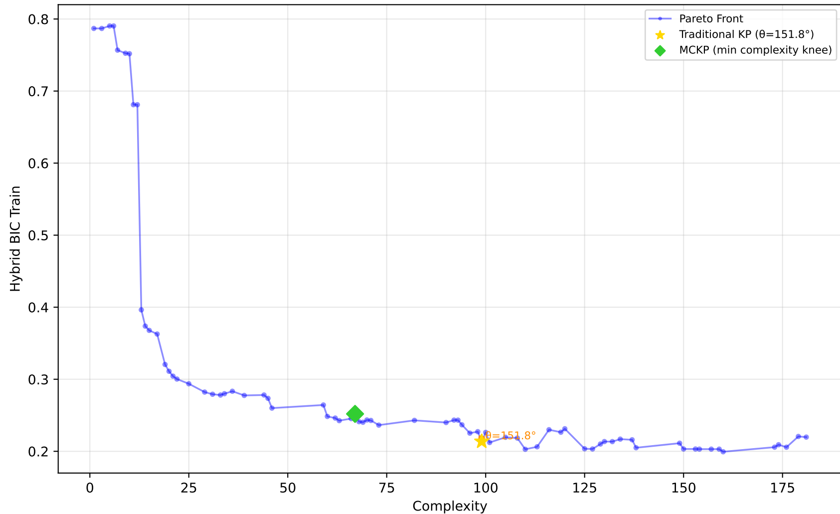
557_analcatdata_apnea1 - Run 26 - SVP - Hybrid BIC Train \lambda_1=0.00, \lambda_2=0.00, \lambda_3=0.00 | Difficulty: 1.00 | Method: hmr
