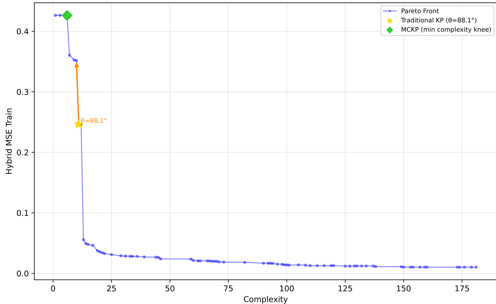
557_analcatdata_apnea1 - Run 26 - SVP - Hybrid MSE Train \lambda_1=0.00, \lambda_2=0.00, \lambda_3=0.00 | Difficulty: 1.00 | Method: hmr
