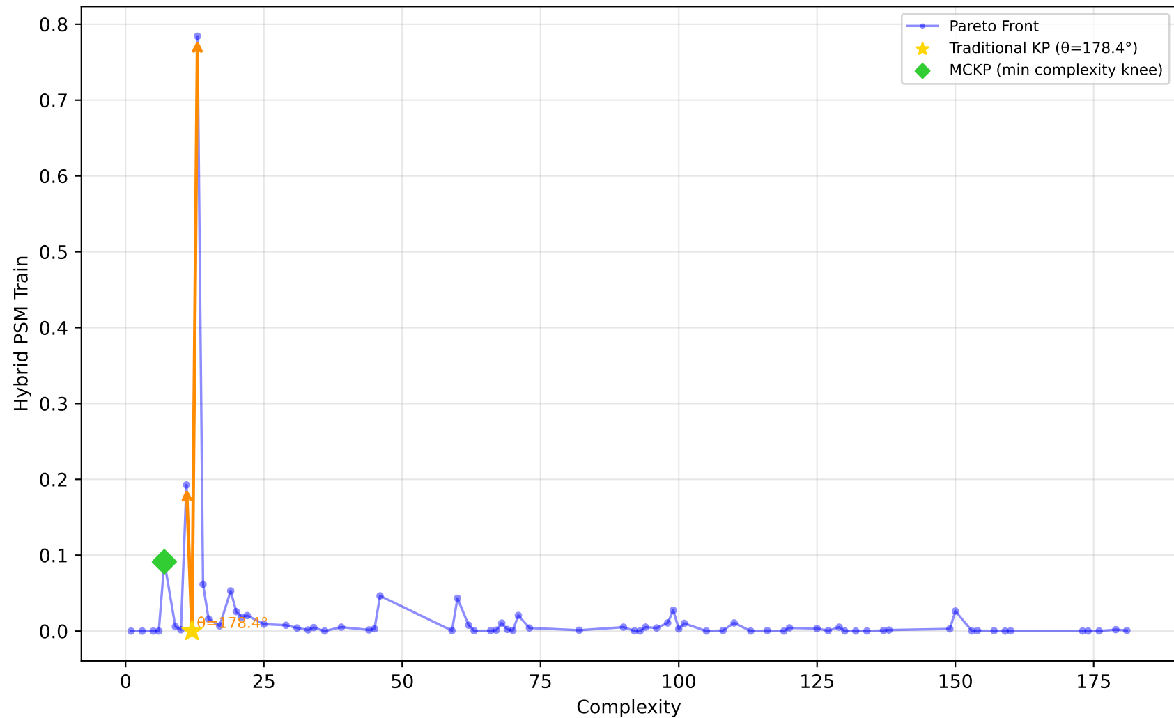
557_analcatdata_apnea1 - Run 26 - SVP - Hybrid PSM Train \lambda_1=0.00, \lambda_2=0.00, \lambda_3=0.00 | Difficulty: 1.00 | Method: hmr
