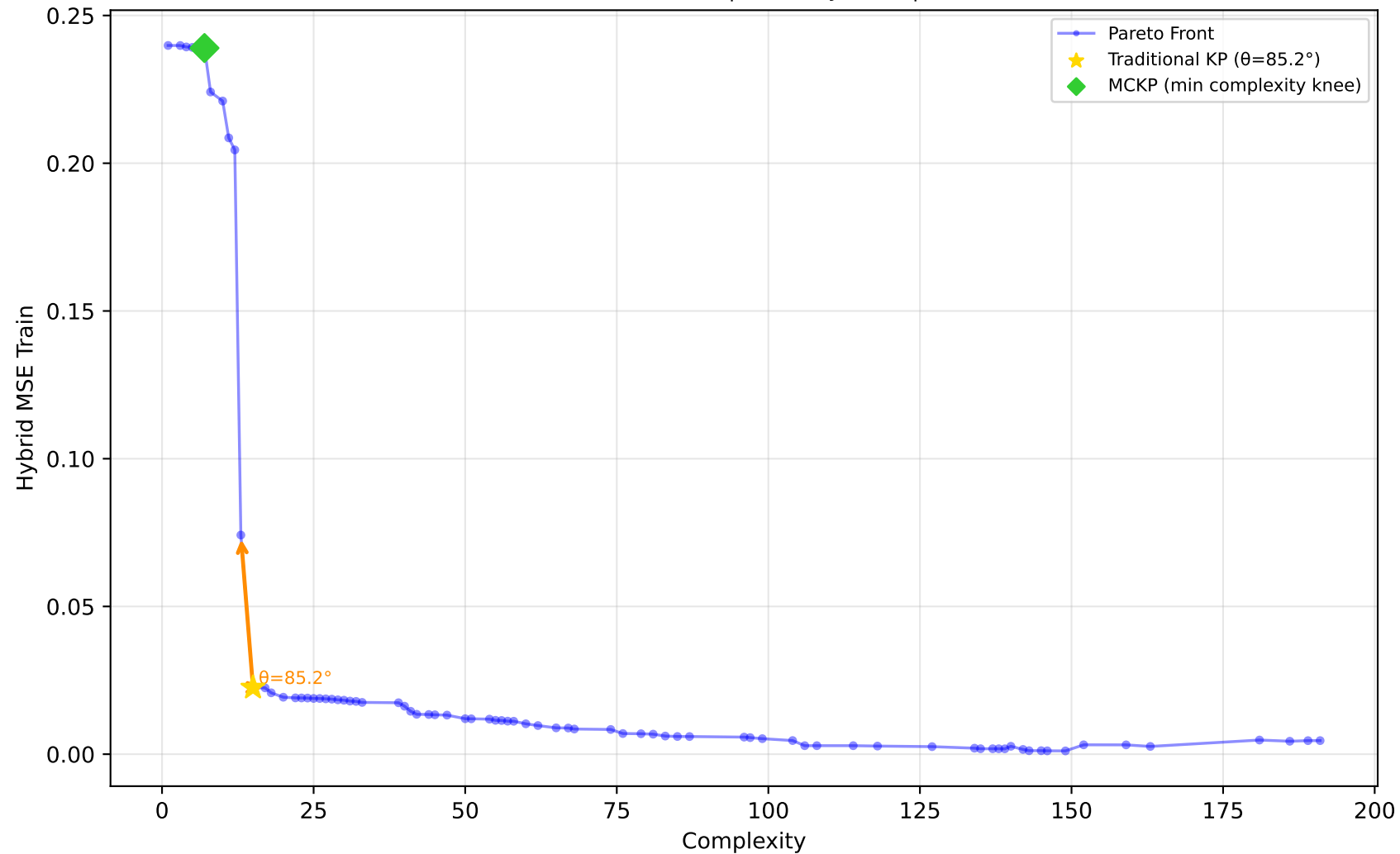
557_analcatdata_apnea1 - Run 27 - MVP - Hybrid MSE Train \lambda_1=0.00, \lambda_2=0.00, \lambda_3=0.00 | Difficulty: 1.00 | Method: hmr
