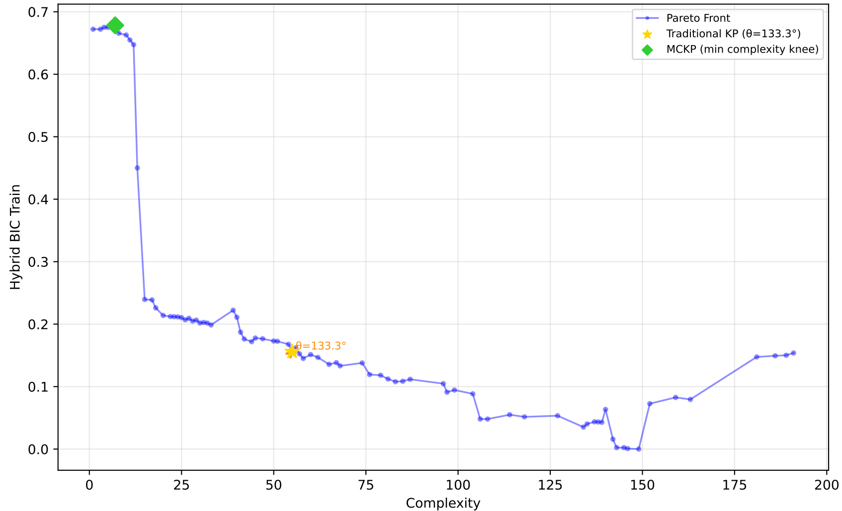
557_analcatdata_apnea1 - Run 27 - SVP - Hybrid BIC Train \lambda_1=0.00 , \lambda_2=0.00 , \lambda_3=0.00 | Difficulty: 1.00 | Method: hmr
