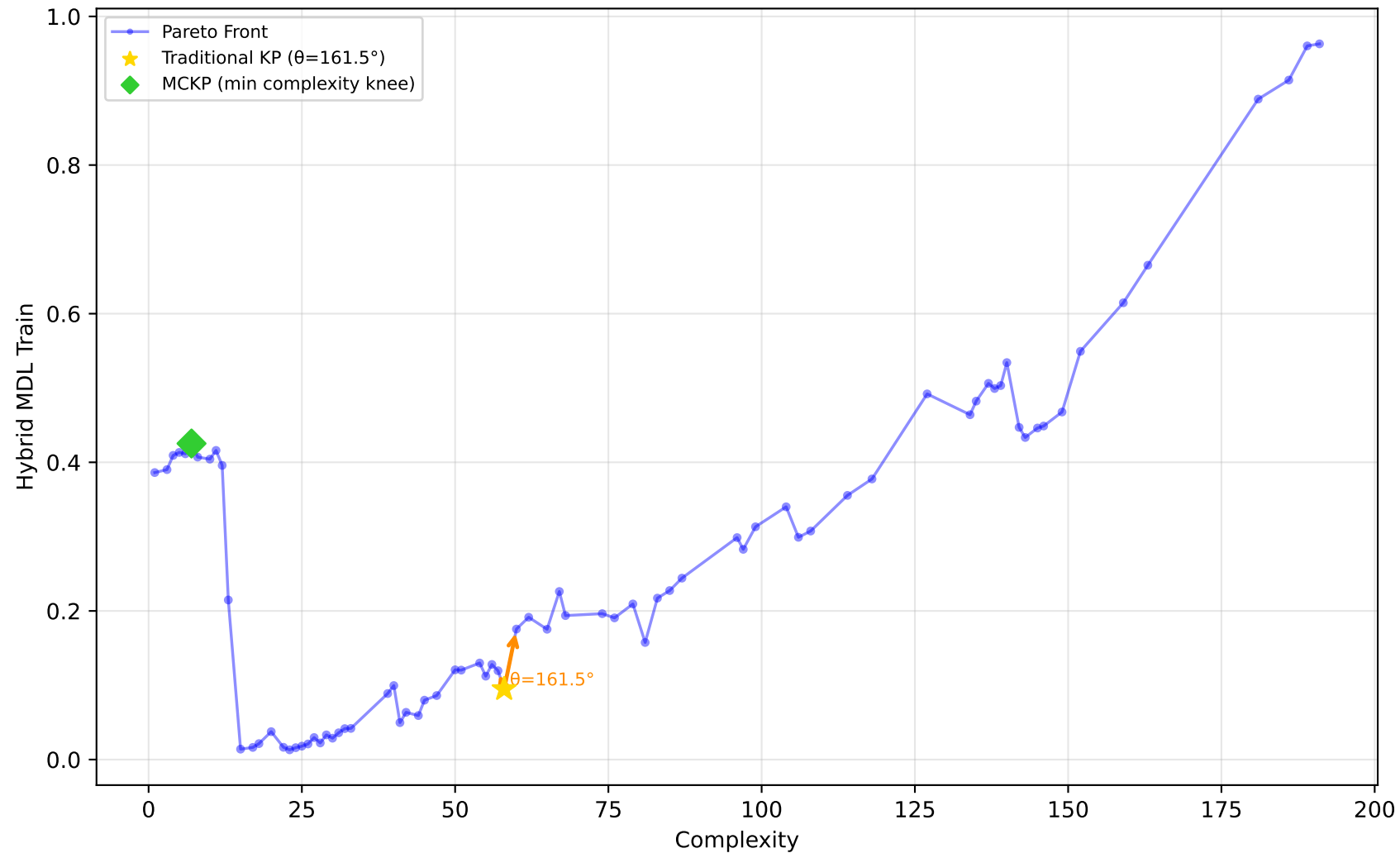
557_analcatdata_apnea1 - Run 27 - SVP - Hybrid MDL Train \lambda_1=0.00 , \lambda_2=0.00 , \lambda_3=0.00 | Difficulty: 1.00 | Method: hmr
