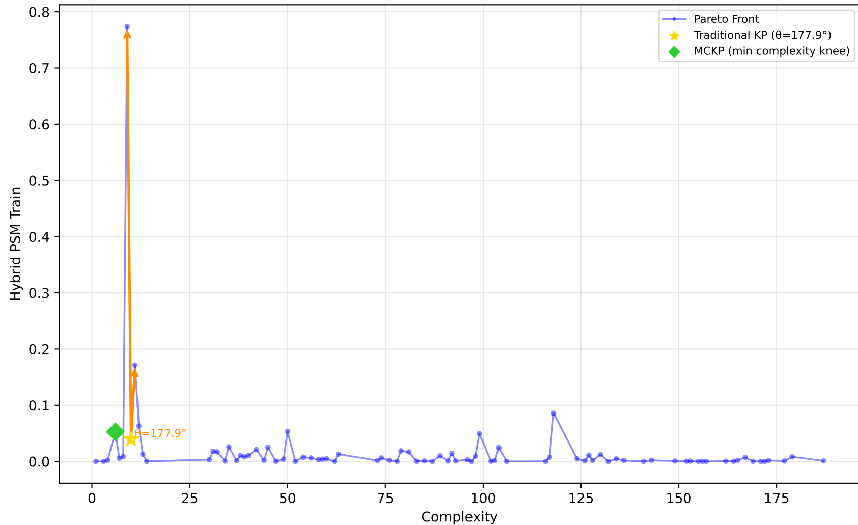
557_analcatdata_apnea1 - Run 28 - MVP - Hybrid PSM Train \lambda_1=0.00, \lambda_2=0.00, \lambda_3=0.00 | Difficulty: 0.66 | Method: hmr
