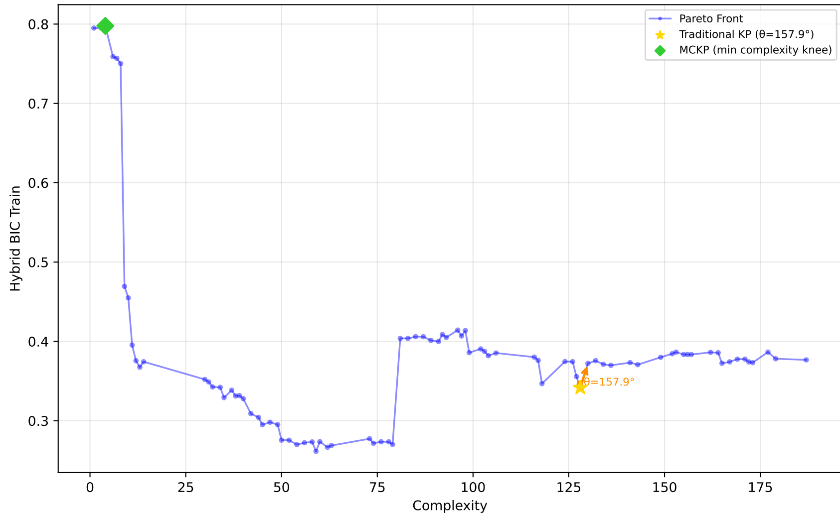
557_analcatdata_apnea1 - Run 28 - SVP - Hybrid BIC Train \lambda_1=0.00, \lambda_2=0.00, \lambda_3=0.00 | Difficulty: 0.66 | Method: hmr
