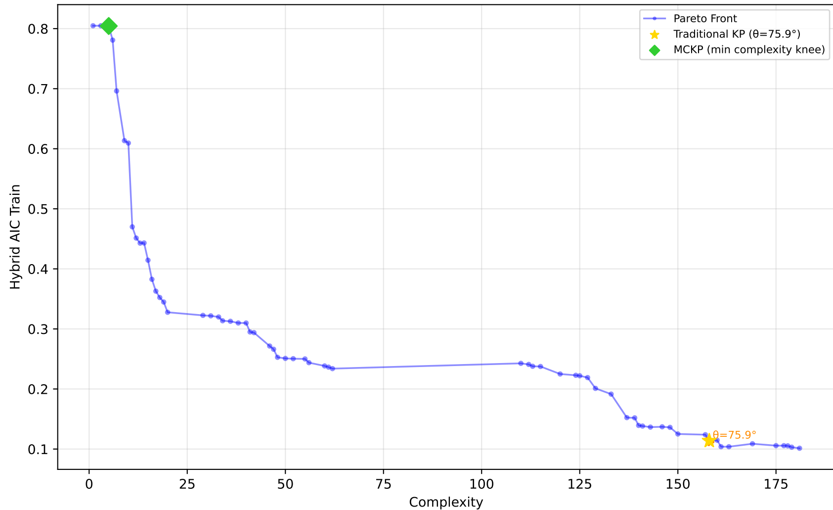
557_analcatdata_apnea1 - Run 29 - MVP - Hybrid AIC Train \lambda_1=0.00, \lambda_2=0.00, \lambda_3=0.00 | Difficulty: 1.00 | Method: hmr
