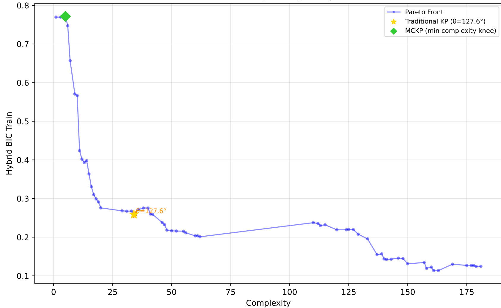
557_analcatdata_apnea1 - Run 29 - MVP - Hybrid BIC Train \lambda_1=0.00, \lambda_2=0.00, \lambda_3=0.00 | Difficulty: 1.00 | Method: hmr
