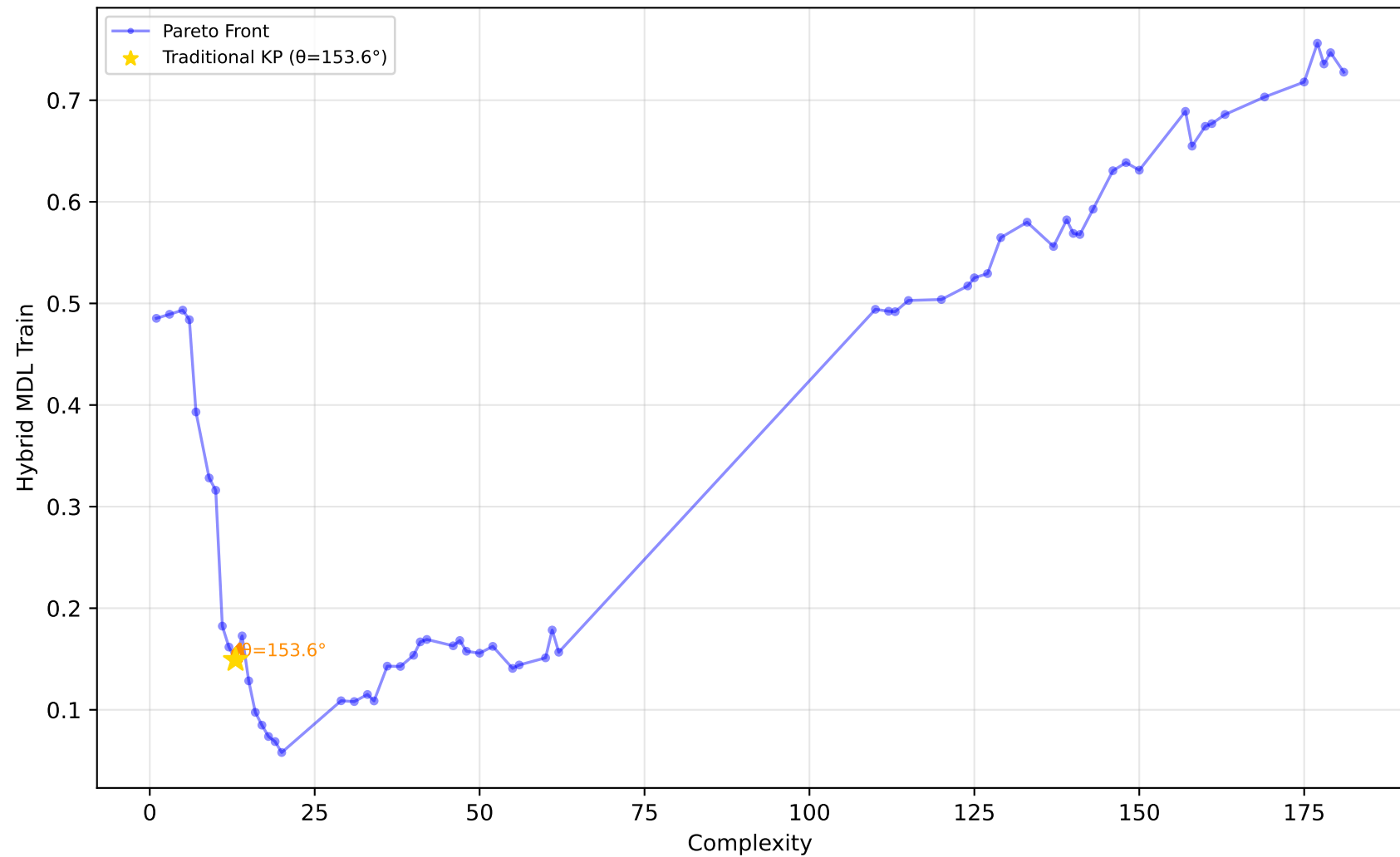
557_analcatdata_apnea1 - Run 29 - MVP - Hybrid MDL Train \lambda_1=0.00, \lambda_2=0.00, \lambda_3=0.00 | Difficulty: 1.00 | Method: hmr
