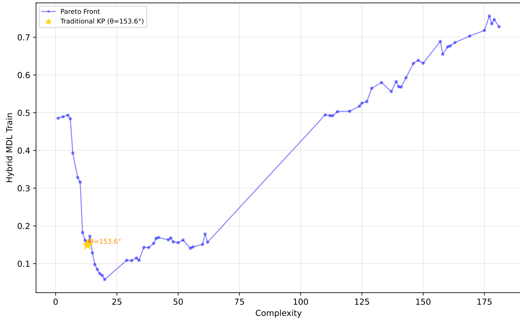
557_analcatdata_apnea1 - Run 29 - SVP - Hybrid MDL Train \lambda_1=0.00, \lambda_2=0.00, \lambda_3=0.00 | Difficulty: 1.00 | Method: hmr
