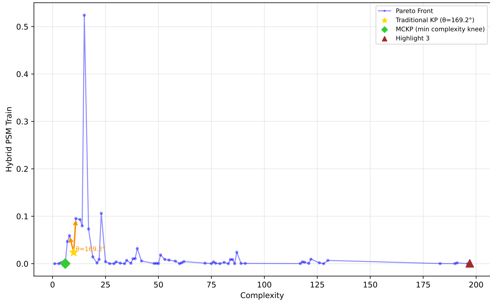
557_analcatdata_apnea1 - Run 2 - MVP - Hybrid PSM Train \lambda_1=0.00, \lambda_2=0.00, \lambda_3=0.00 | Difficulty: 1.00 | Method: hmr
