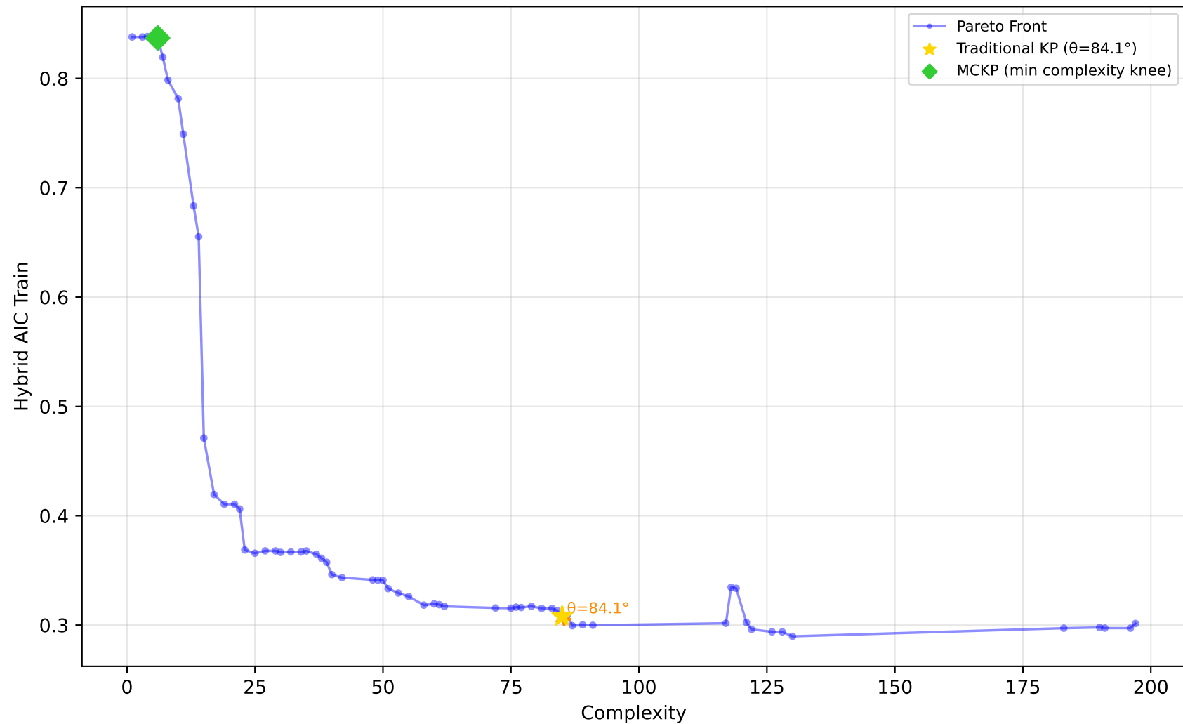
557_analcatdata_apnea1 - Run 2 - SVP - Hybrid AIC Train \lambda_1=0.00, \lambda_2=0.00, \lambda_3=0.00 | Difficulty: 1.00 | Method: hmr
