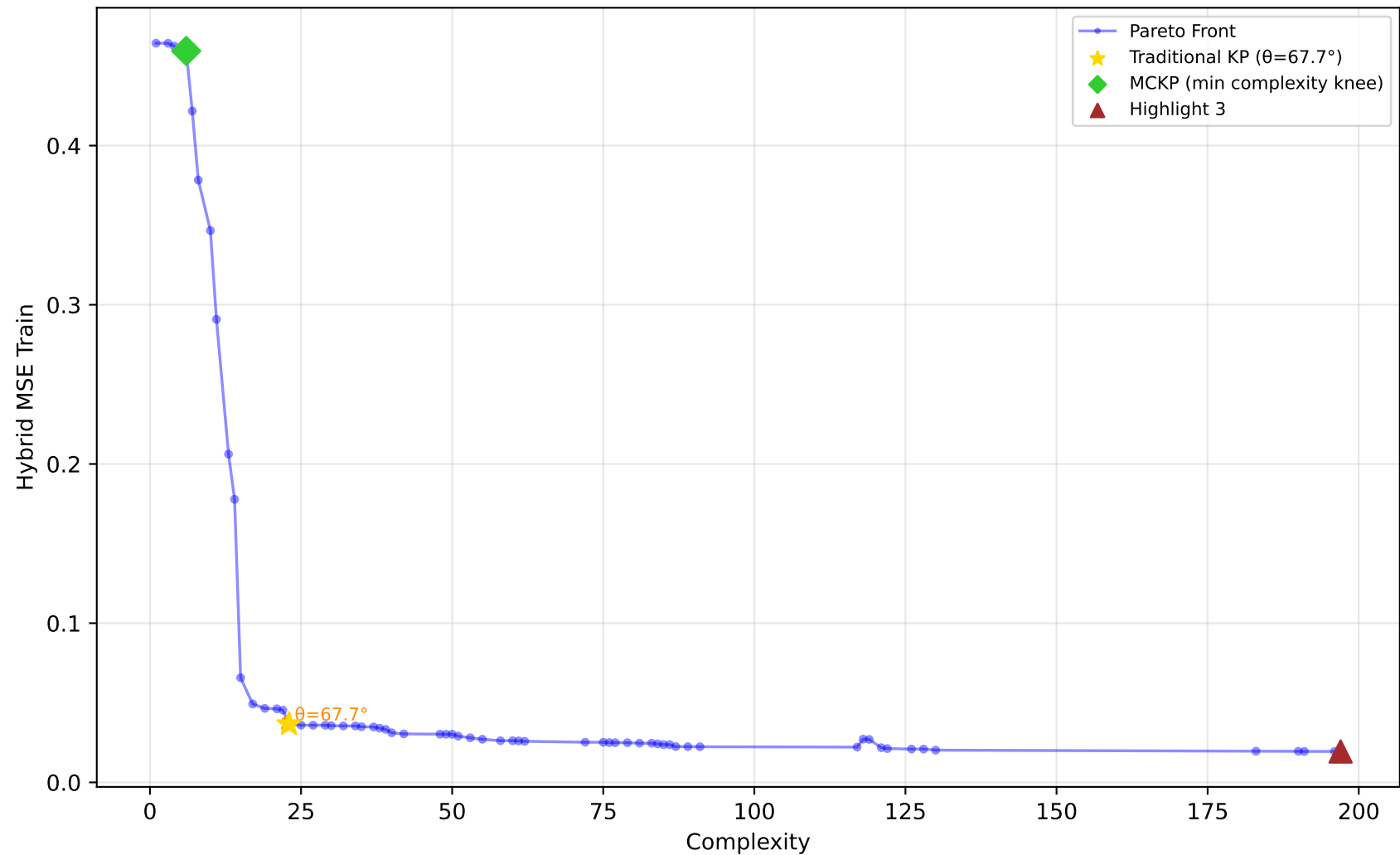
557_analcatdata_apnea1 - Run 2 - SVP - Hybrid MSE Train \lambda_1=0.00, \lambda_2=0.00, \lambda_3=0.00 | Difficulty: 1.00 | Method: hmr
