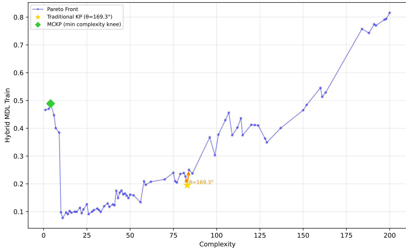
557_analcatdata_apnea1 - Run 30 - MVP - Hybrid MDL Train \lambda_1=0.00, \lambda_2=0.00, \lambda_3=0.00 | Difficulty: 1.00 | Method: hmr
