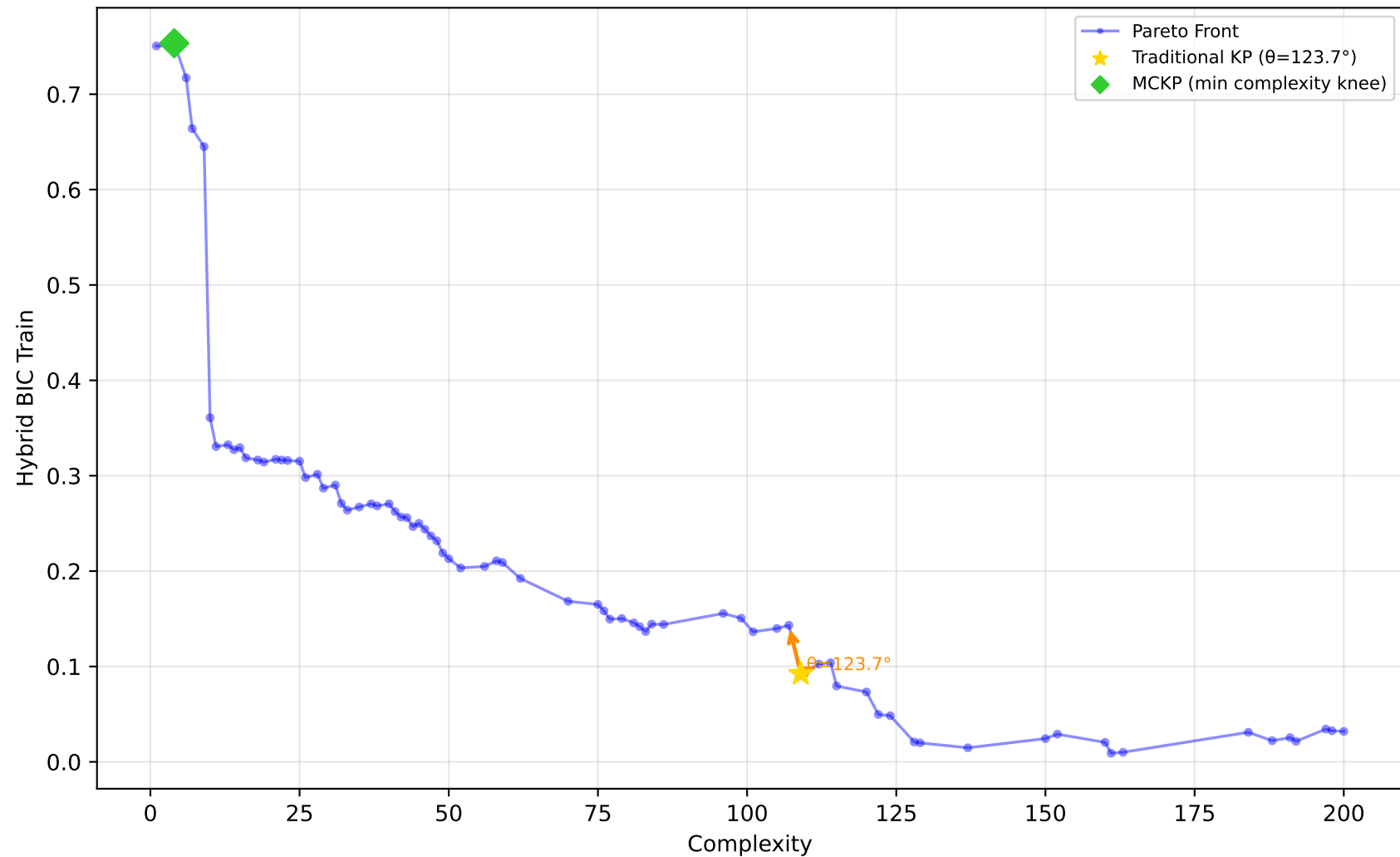
557_analcatdata_apnea1 - Run 30 - SVP - Hybrid BIC Train \lambda_1=0.00, \lambda_2=0.00, \lambda_3=0.00 | Difficulty: 1.00 | Method: hmr
