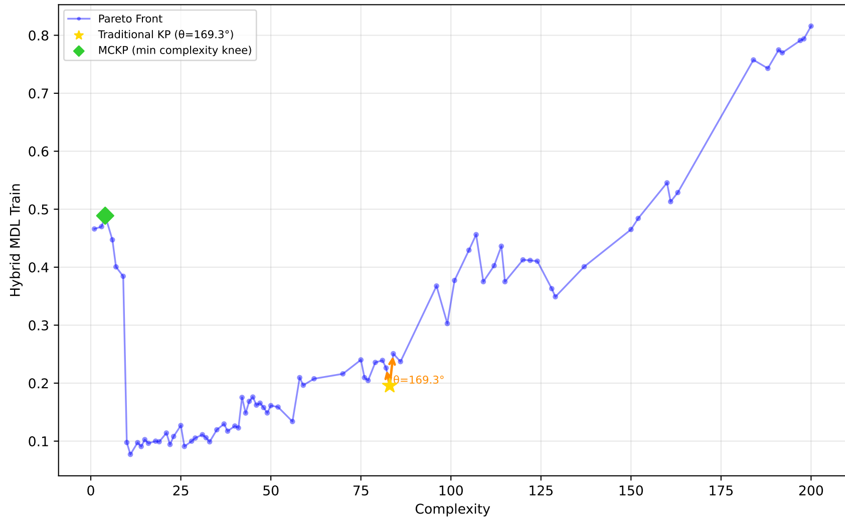
557_analcatdata_apnea1 - Run 30 - SVP - Hybrid MDL Train \lambda_1=0.00, \lambda_2=0.00, \lambda_3=0.00 | Difficulty: 1.00 | Method: hmr
