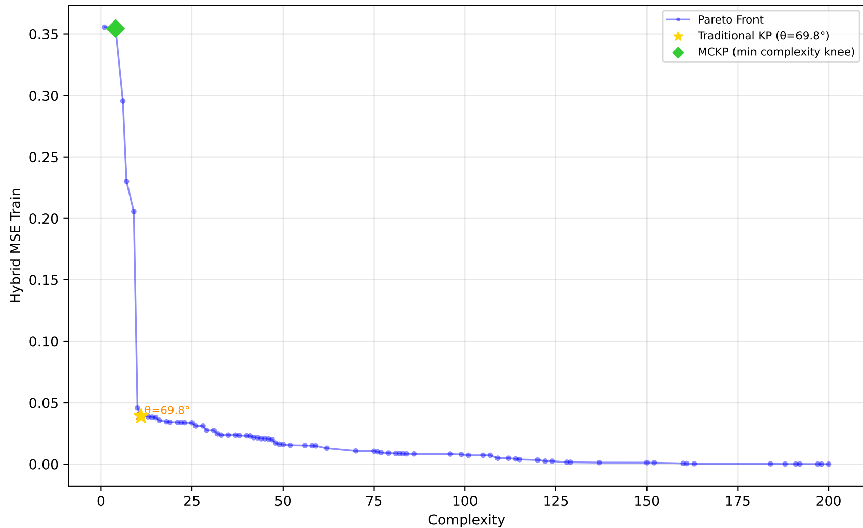
557_analcatdata_apnea1 - Run 30 - SVP - Hybrid MSE Train \lambda_1=0.00 , \lambda_2=0.00 , \lambda_3=0.00 | Difficulty: 1.00 | Method: hmr
